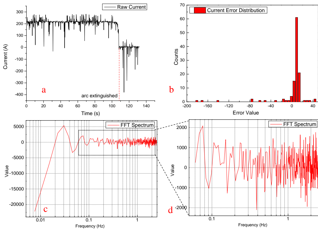
Figure 16a. Raw current signal for a single layer; 16b. error histogram for current data after arc extinguished 16c. fast Fourier Transformed Current Spectrum; 1d. zoom-in diagram of 15c from 0.05Hz;
