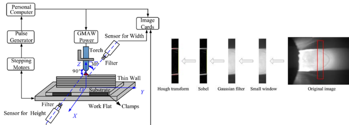
Figure 6 Set-up for layer height & width monitoring (Xiong et al. 2016)
