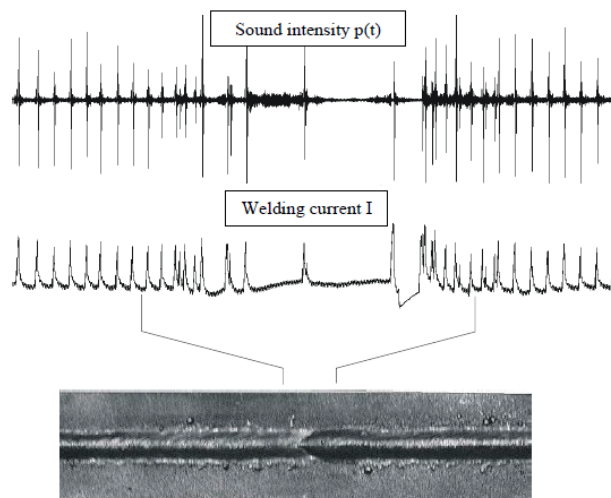
Figure 3 Integrated Process parameters monitoring system (Polajnar et al. 2013)
