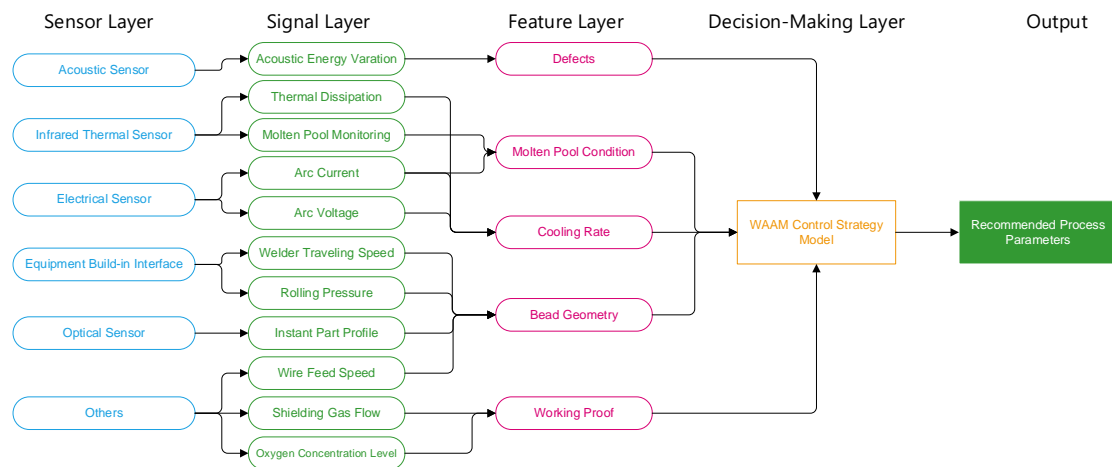
Figure 8 Schematic diagram of Full State Monitoring System for WAAM
